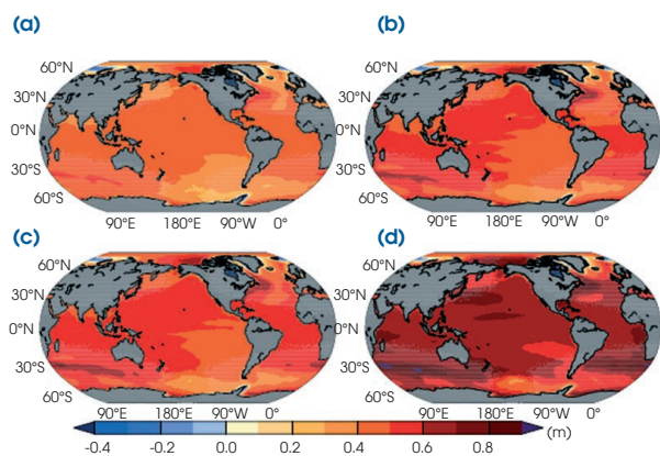
Fig.3 — Overall average (21 CMIP5 models) of the change in relative sea level for RCP2.6 scenarios (a), 4.5 (b), 6.0 (c) and 8.5 (d). The impact of thermal expansion of the oceans, the mass of continental ice, continental stocks of liquid water and post-glacial rebound have been taken into account (adapted from Church et al. , 2013).
